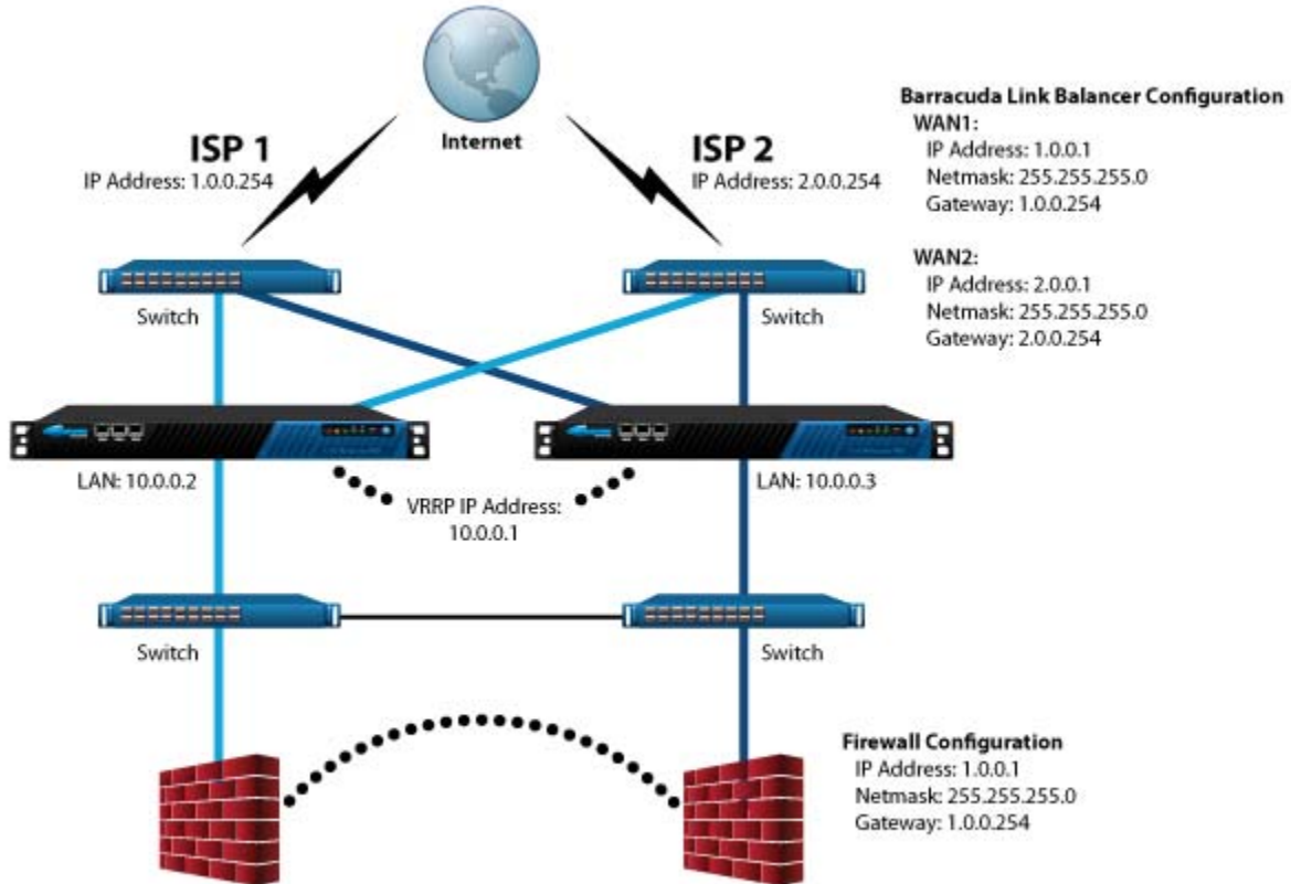
Figure 4.4: Deployment Example - Dual Firewalls
