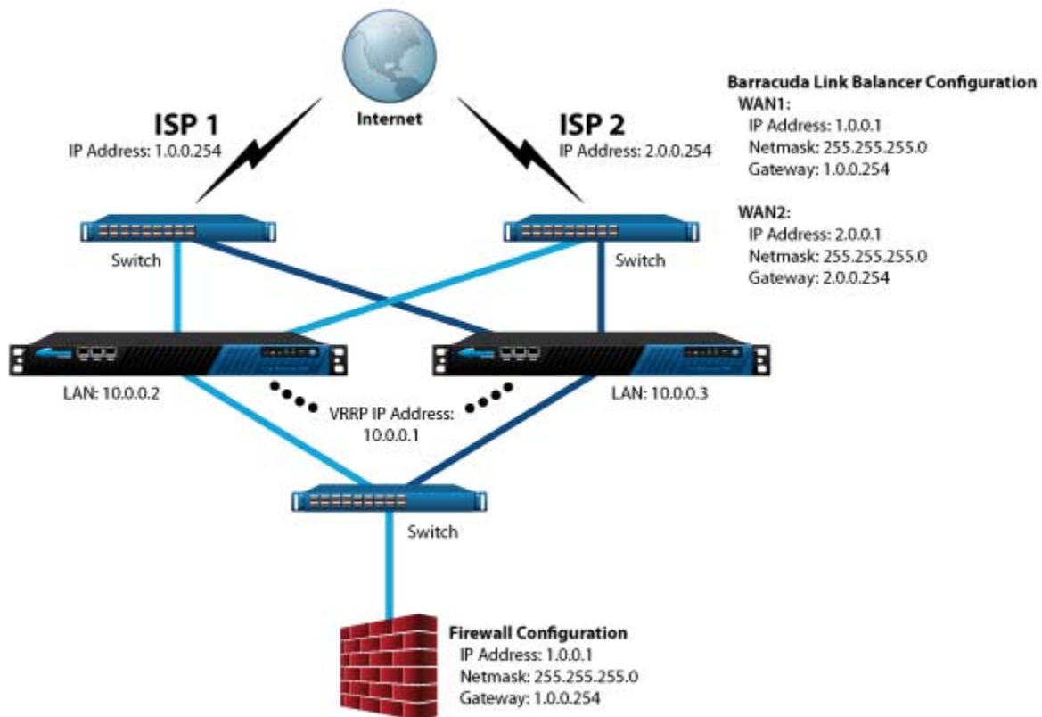
Figure 4.3: Deployment Example - Single Firewall
